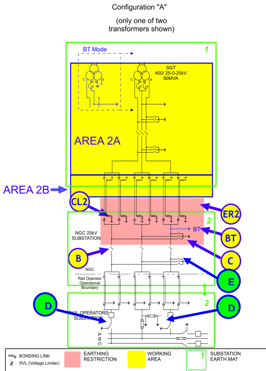
Figure 4.4 An example of Point(s) of Isolation on the neutral conductor only.
