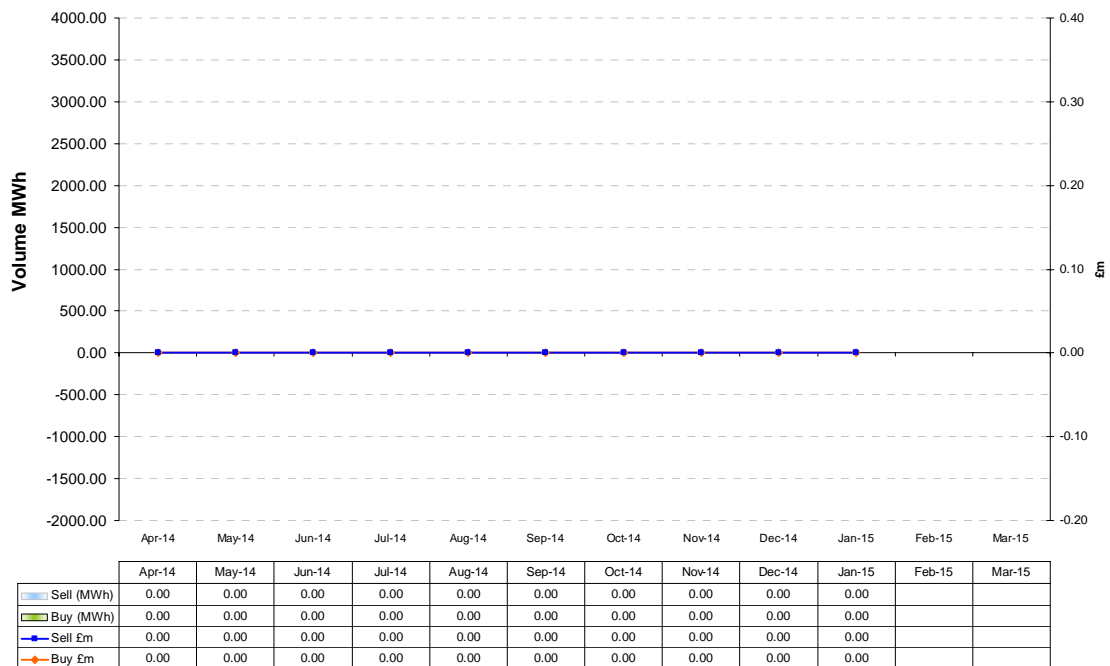
PGBT Actions
