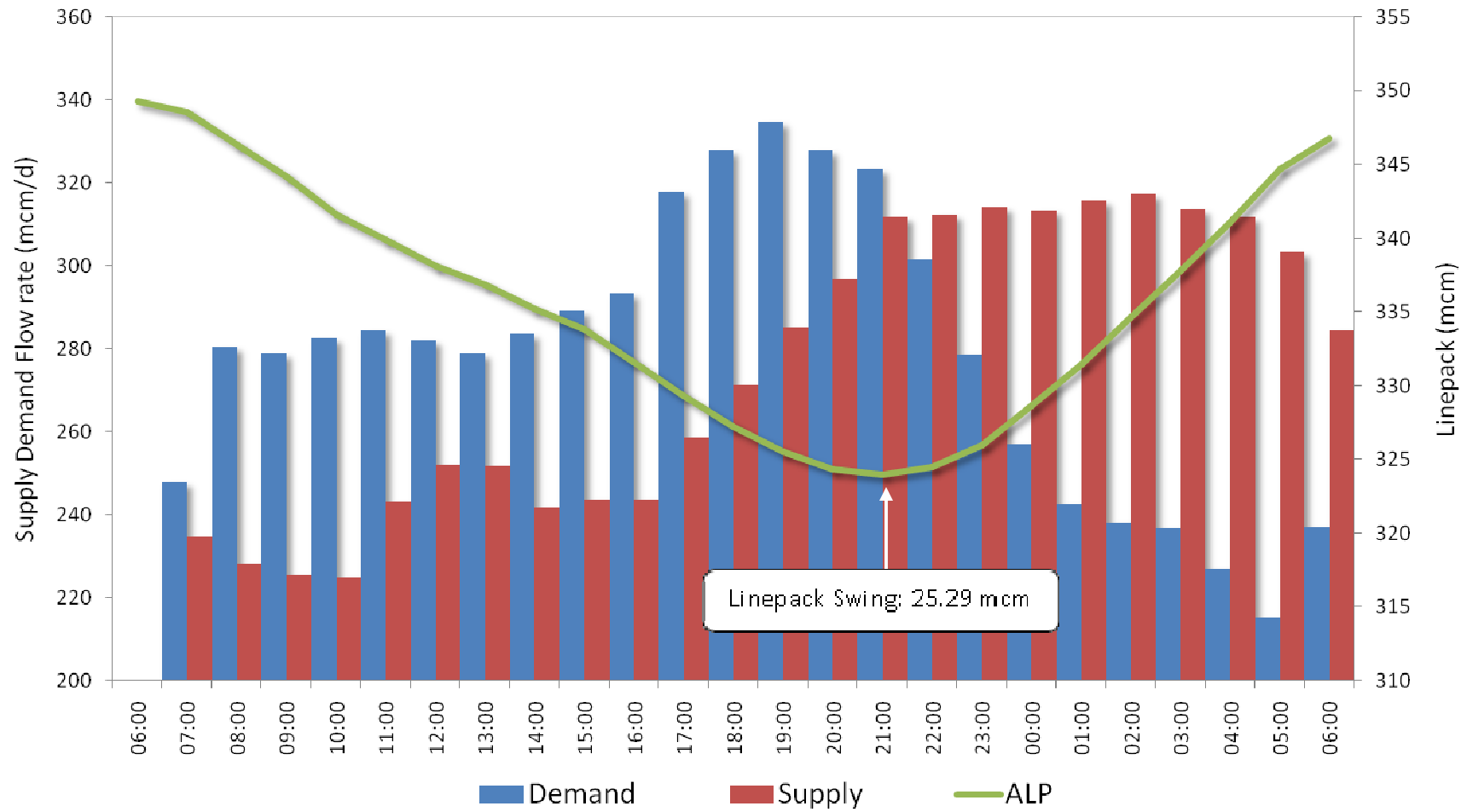
Supply and Demand Flow Profiles vs Actual Linepack
