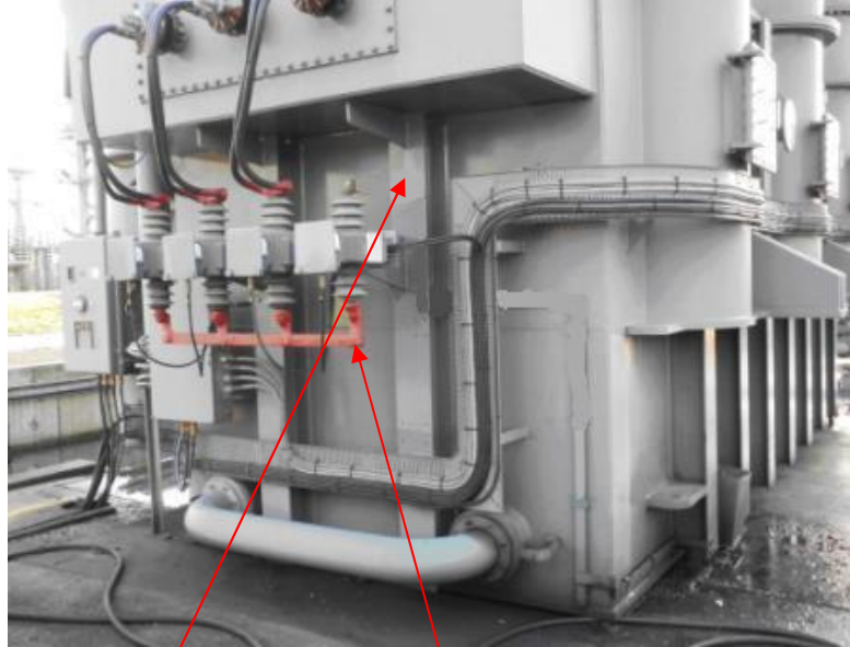
Figure 7.2b - Defective or missing neutral earth connections between the Equipment star point and the Main Earth System
