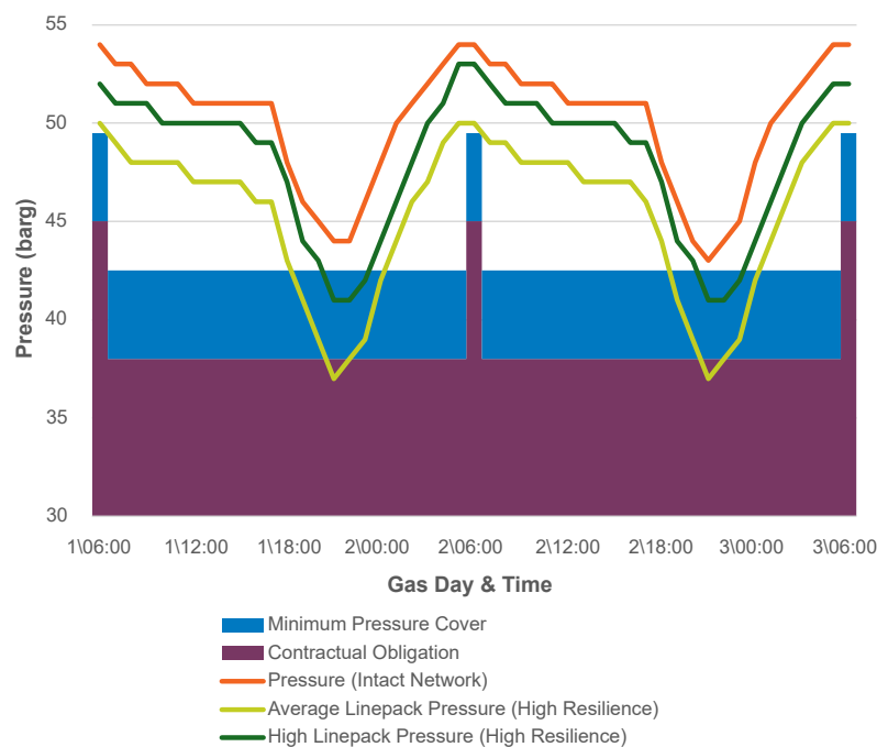
Figure 5: NTS South East Pressure (1 Hour Ramp Rate)
