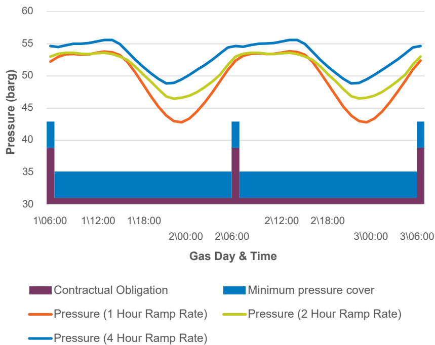
Figure 6: NTS South West Pressure
