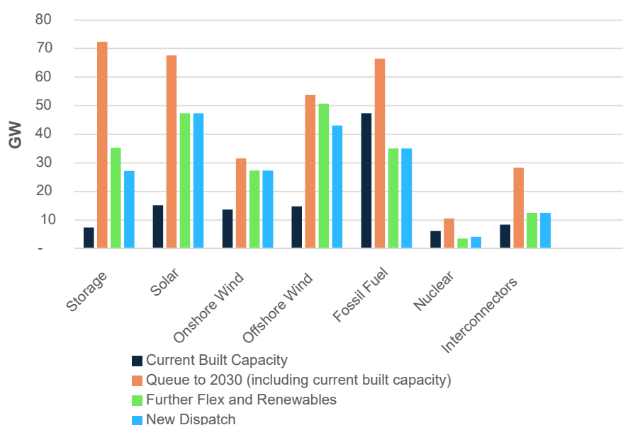
Figure 7: The current unreformed queue, broken down by technology and year out to 2030 alongside each pathway and where the queue stands relative to the requirements of each pathway in 2030
