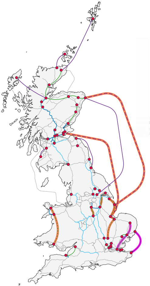
Figure 3: Map of the network recommended for clean power, showing schemes that must be supported back to 2030 (in purple) and schemes that are beneficial if accelerated to 2030 (in red).
