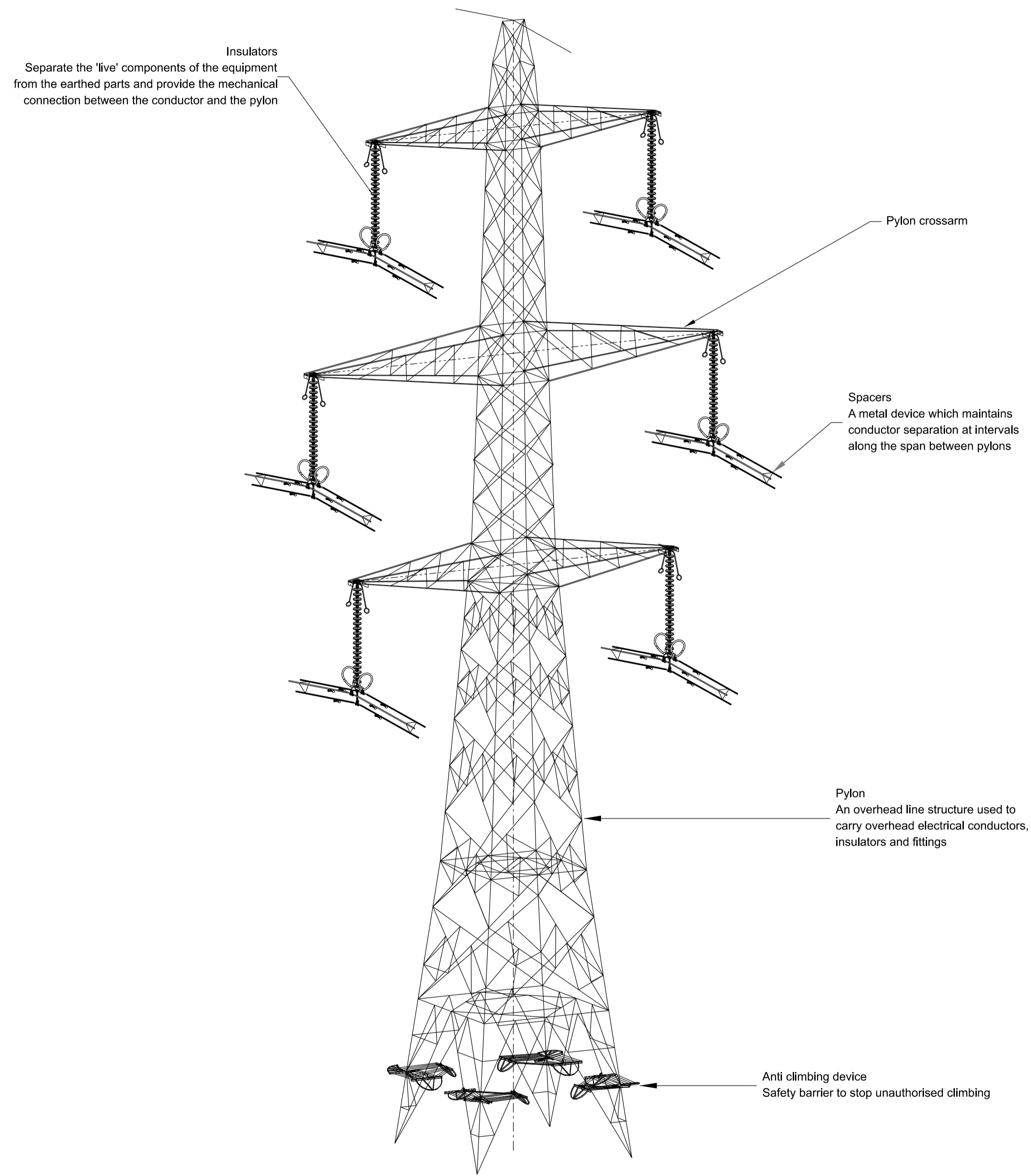
Isometric view on pylon L12 D STD
