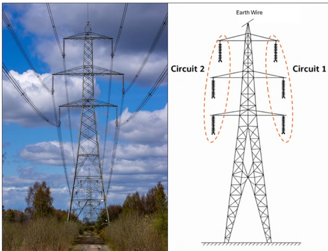
Figure C.1 – Example of a 400 kV Double-circuit Tower
