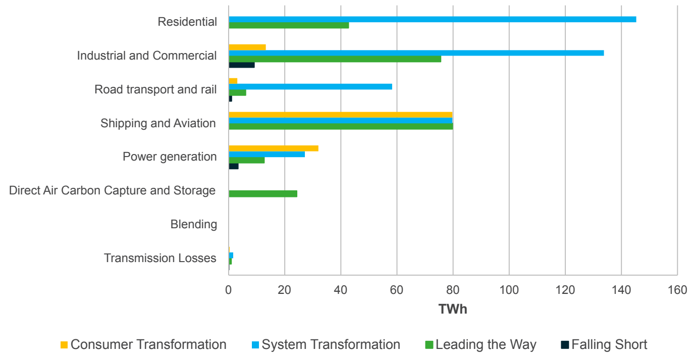
Figure ES.32: Low carbon hydrogen demand
