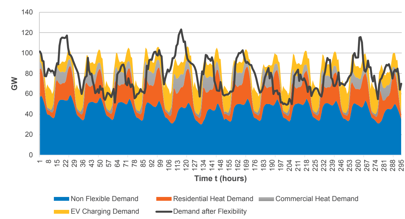
Figure FL.24: Non-flexible demand profiling alongside demand line after flexibility (GWh)
