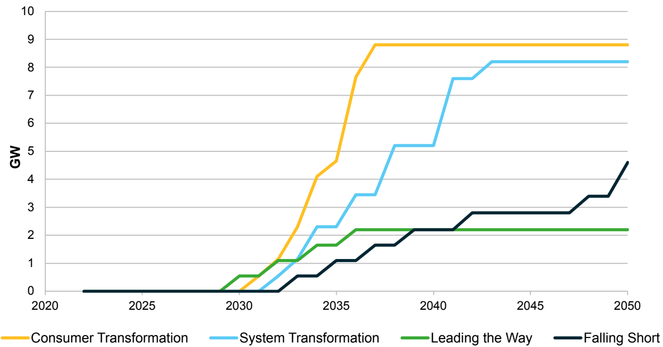
Figure ES.17: BECCS generation capacity in GW
