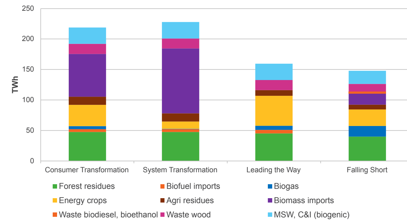
Figure ES.45: Total bioenergy supply in 2050
