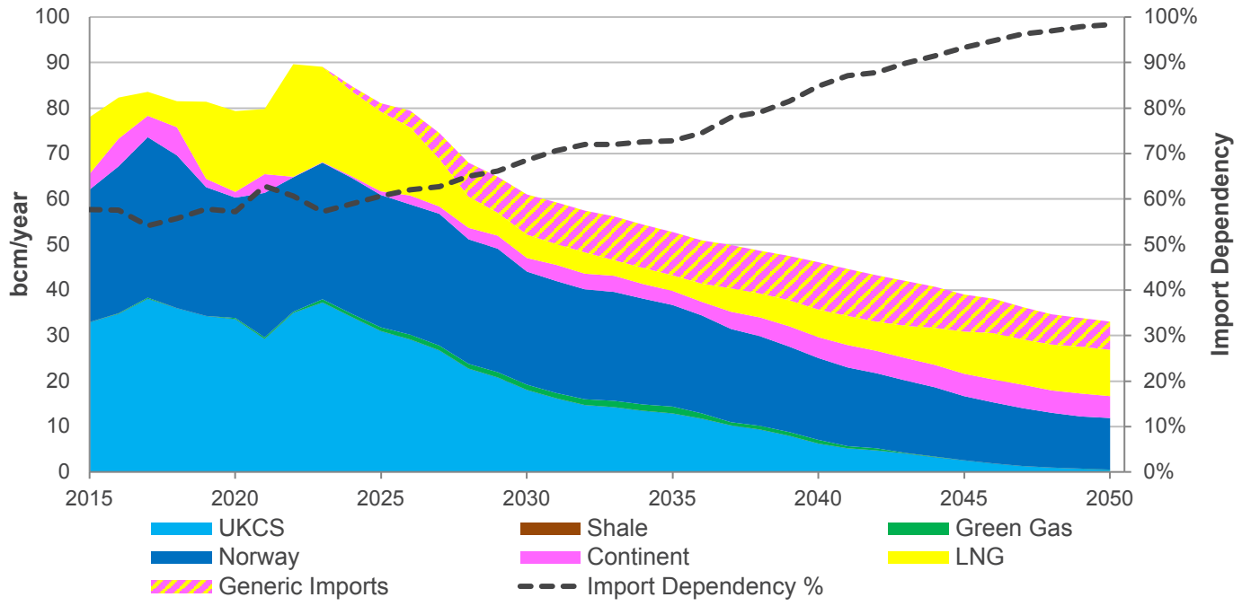
Figure ES.38: Annual gas supply in System Transformation
