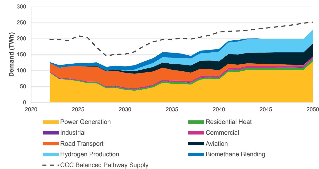
Figure ES.47: Bioenergy demand by sector in System Transformation
