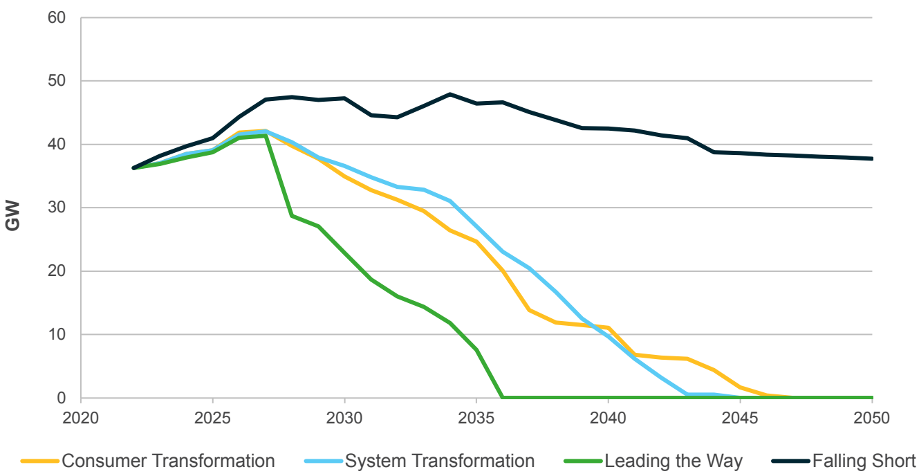
Figure ES.15: Unabated gas capacity in GW
