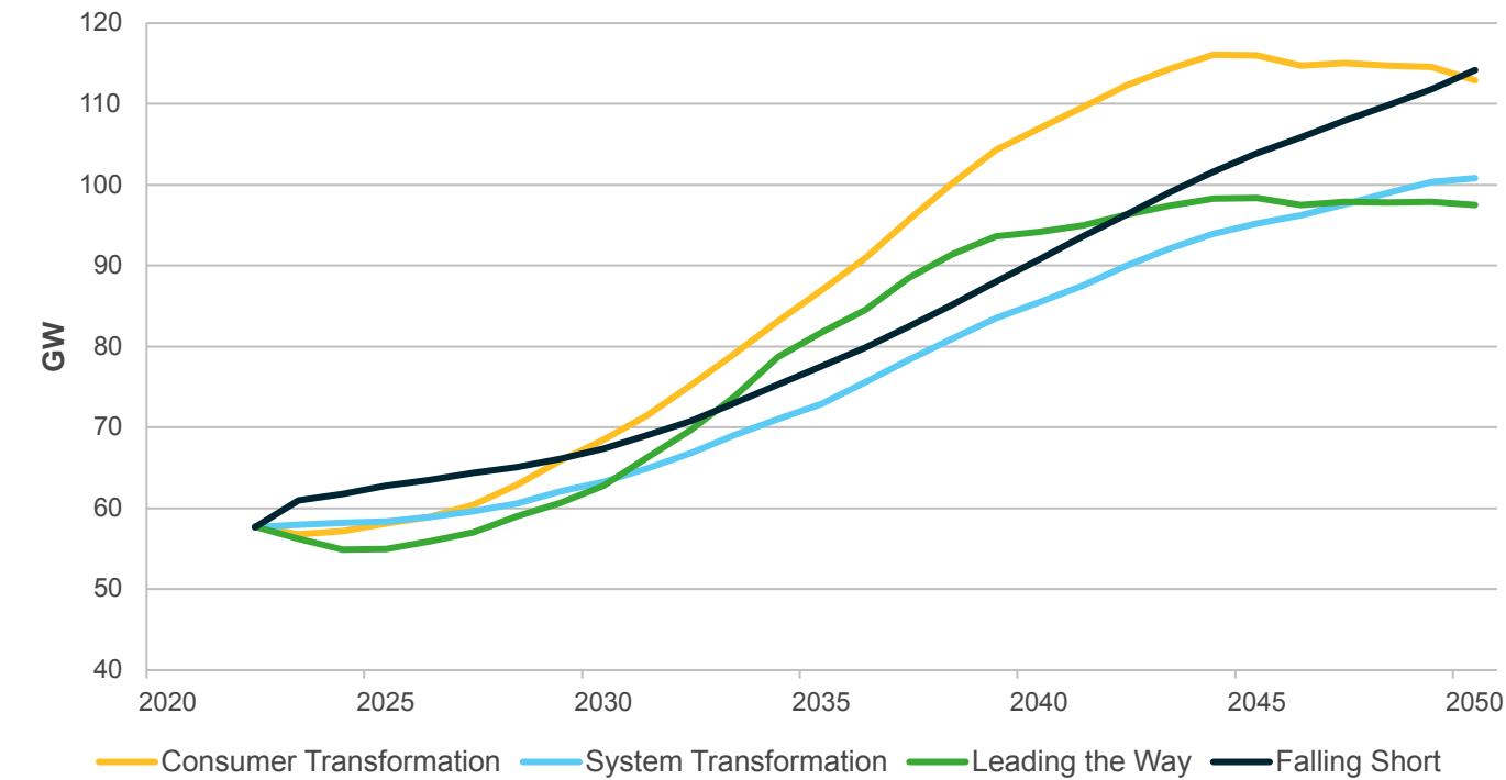
Figure ES.03: ACS Electricity Peak Demand
