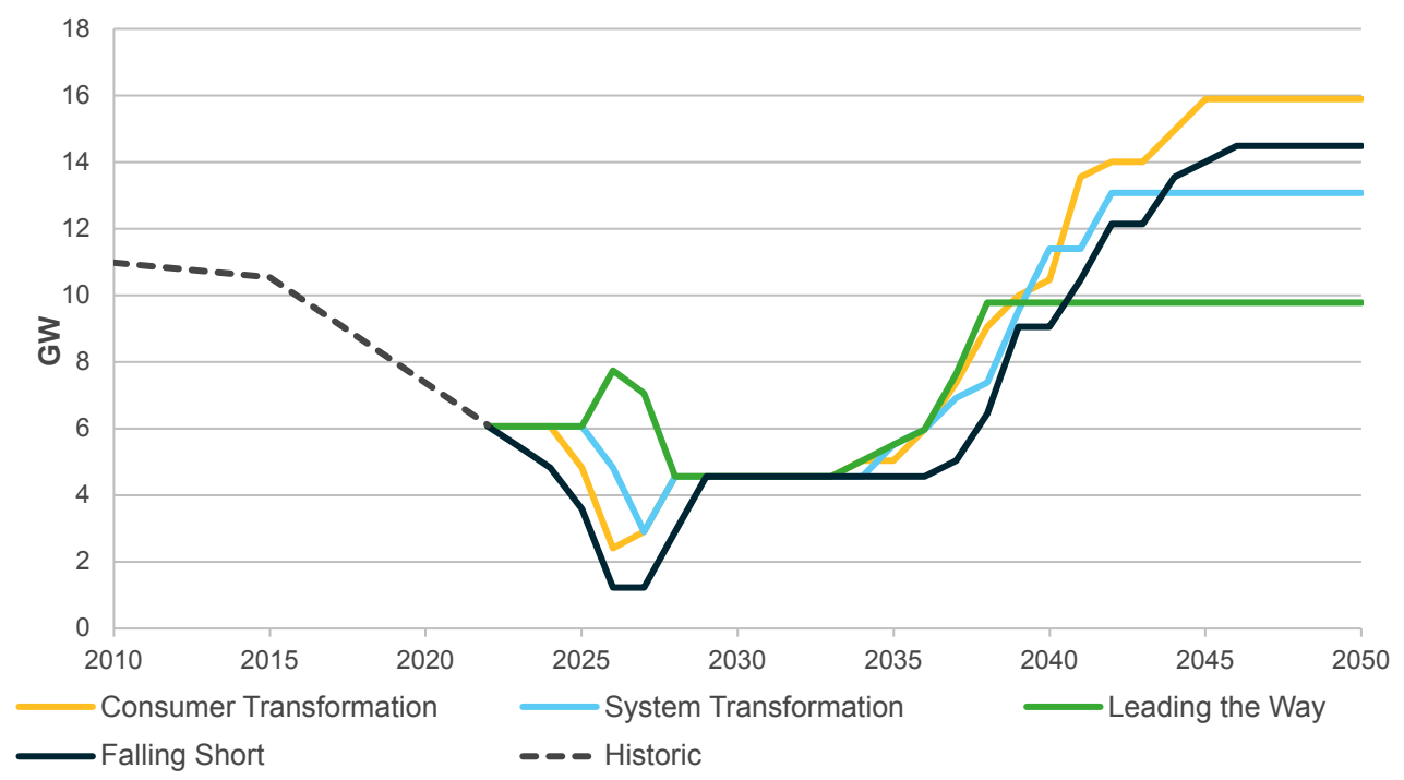
Figure ES.18: Nuclear generation of existing plant
