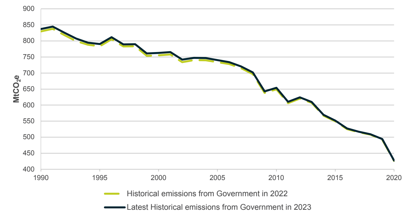
Figure NZ.07: Total net GHG emissions
