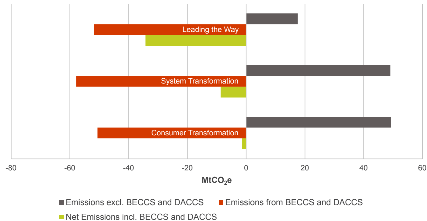
Figure NZ.17: Net annual emissions sensitivity analysis (BECCS and DACCS)
