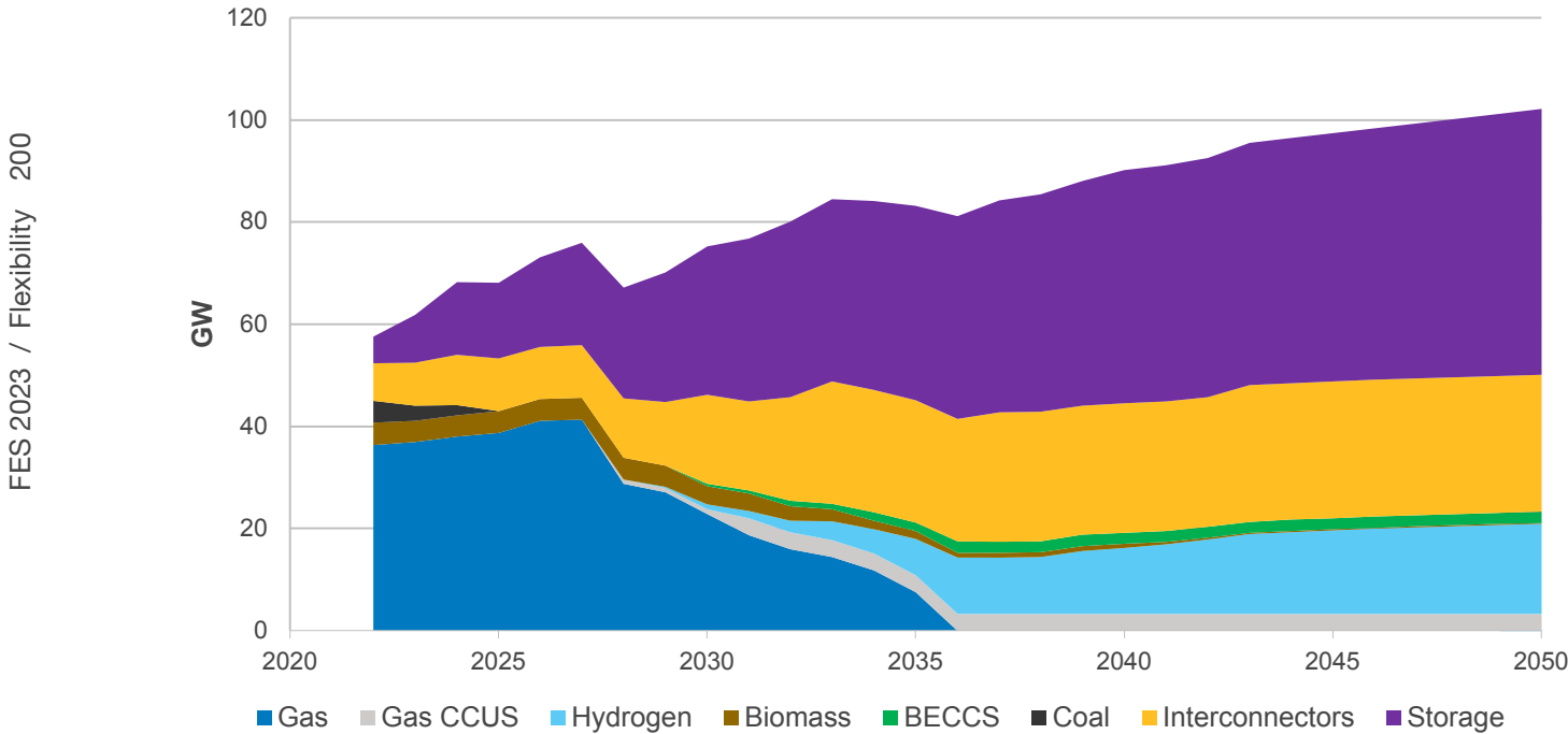
Figure FL.16: Dispatchable electricity supply sources (excluding renewable sources) for Leading the Way
