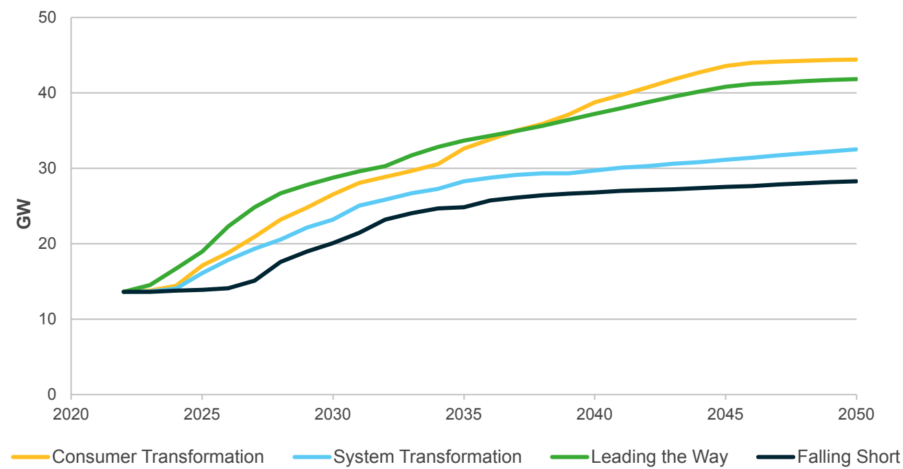
Figure ES.12: Onshore wind capacity in GW
