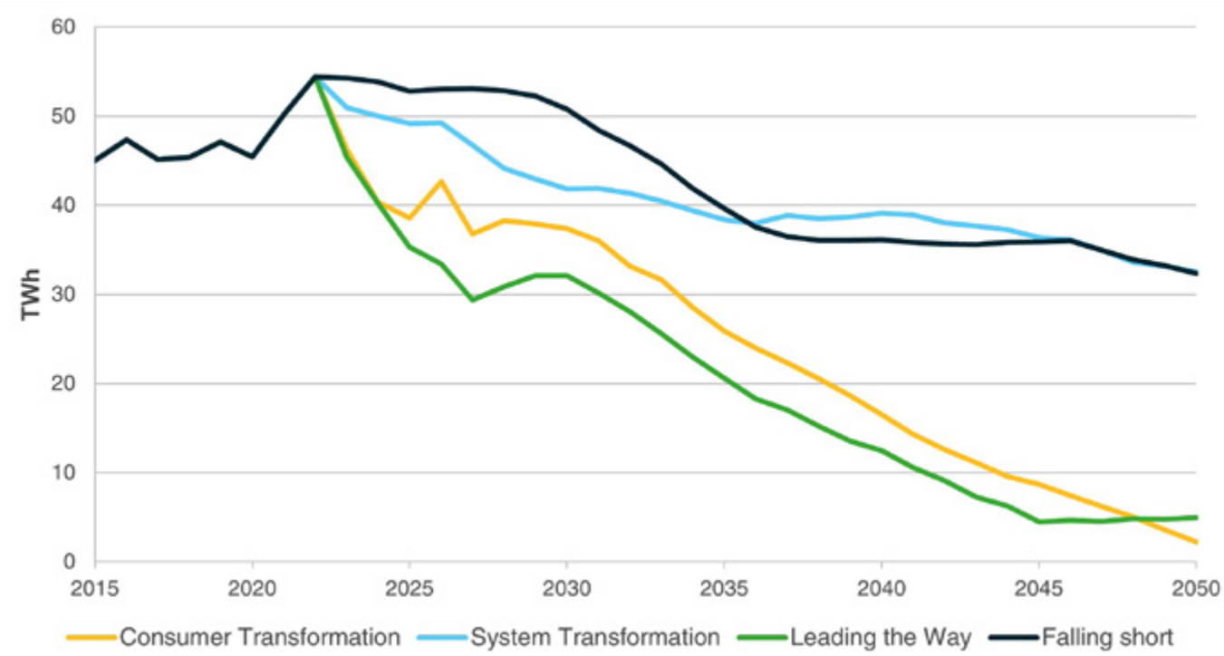
Figure ES.41: Imported gas volumes
