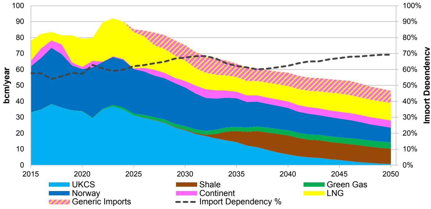
Figure ES.40: Annual gas supply in Falling Short
