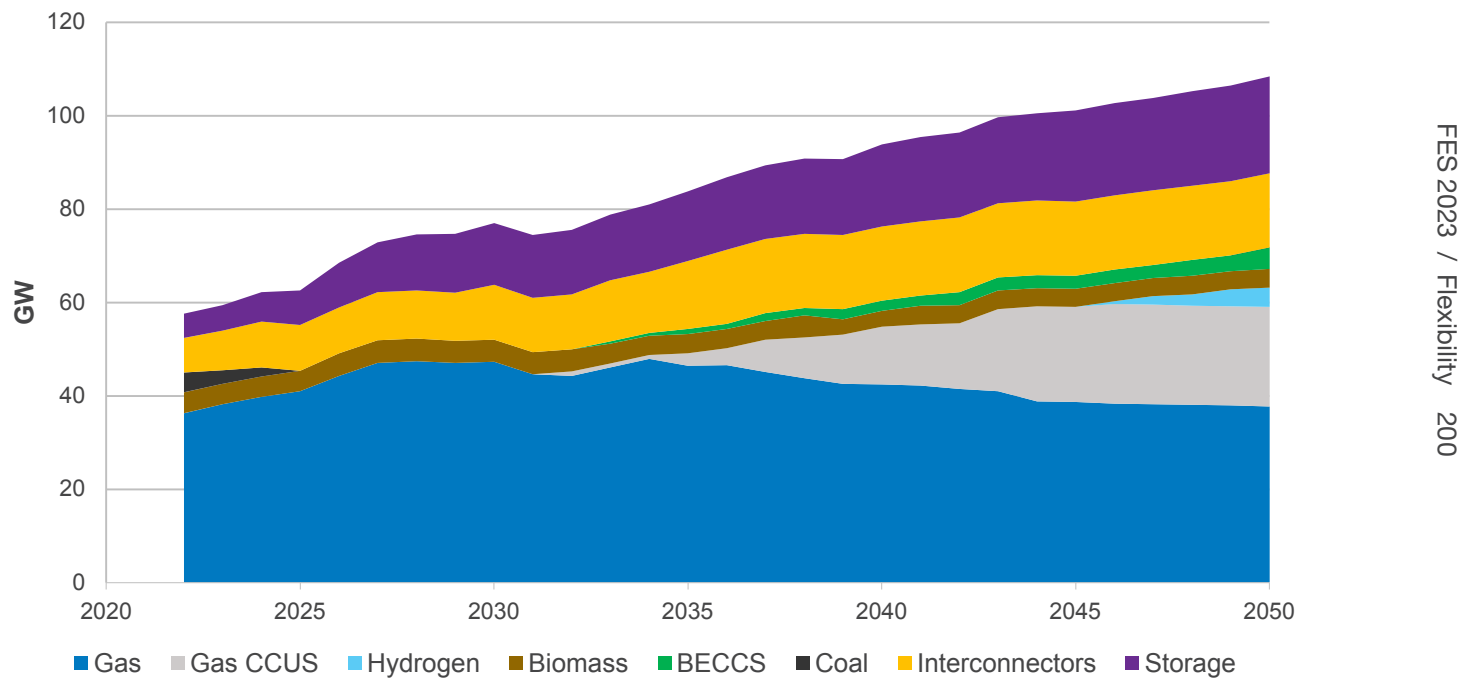
Figure FL.17: Dispatchable electricity supply sources (excluding renewable sources) for Falling Short
