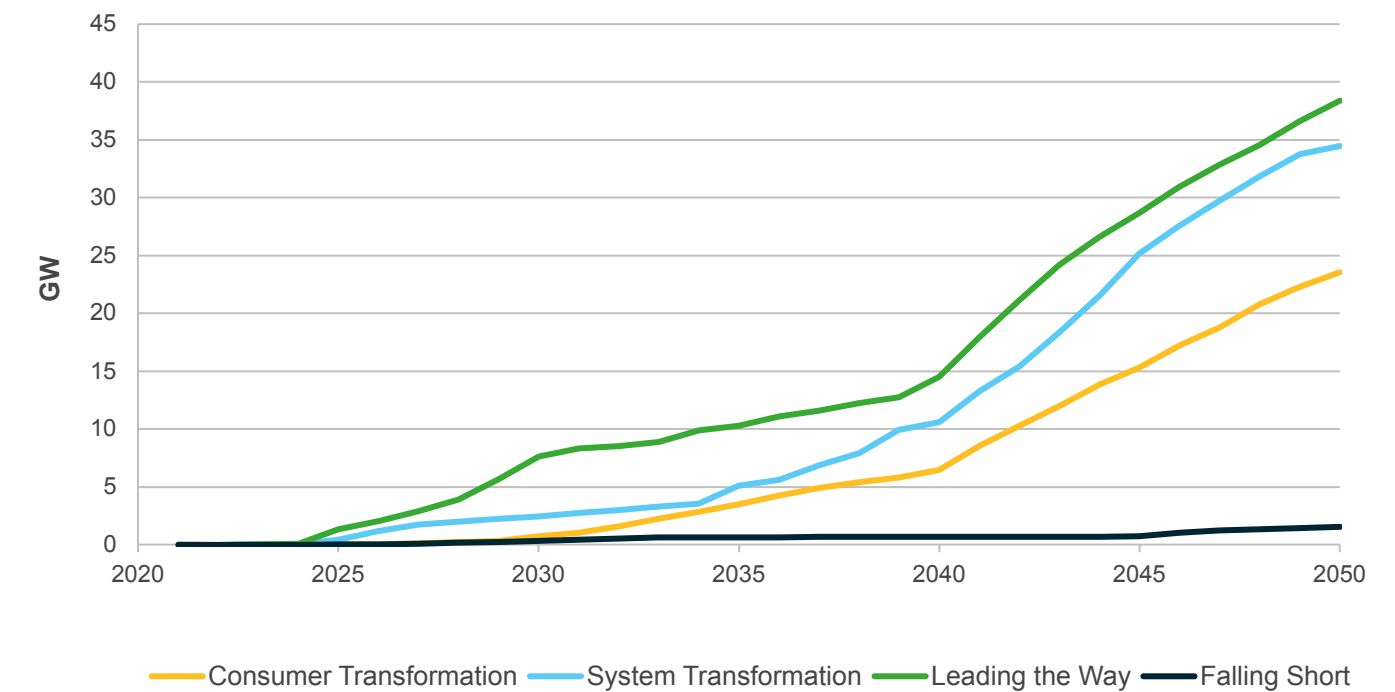
Figure FL.08: Network-connected electrolysis capacity: Electrolyzers connected to the GB distribution and transmission systems either directly or via generation plant (excluding nuclear)
