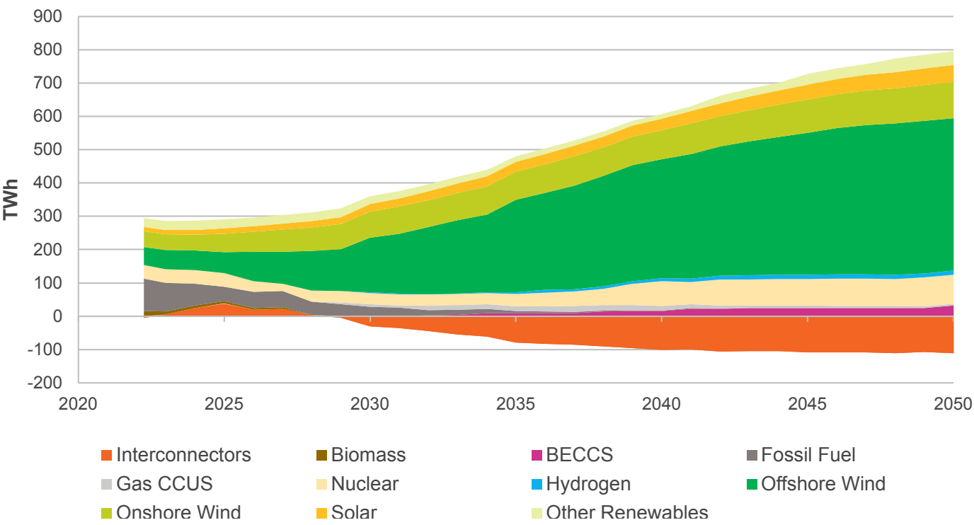
Figure ES.06: Electricity output by technology in System Transformation
