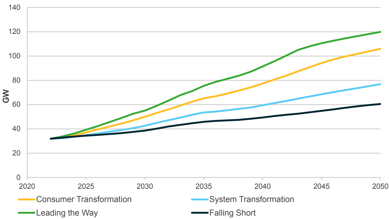
Figure ES.22: Distribution connection generation
