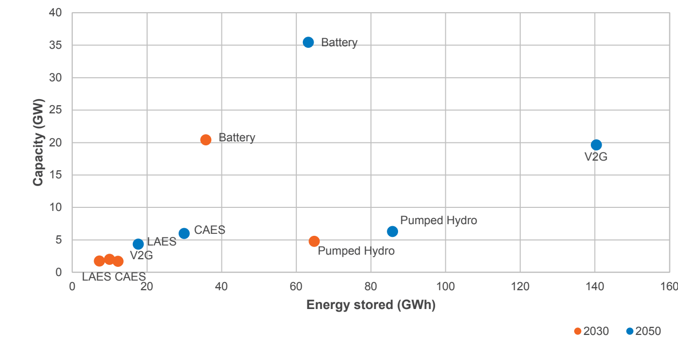
Figure FL.12: Varying energy and power outputs of electricity storage types in 2030 and 2050 for Leading the Way (including Vehicle-to-Grid)
