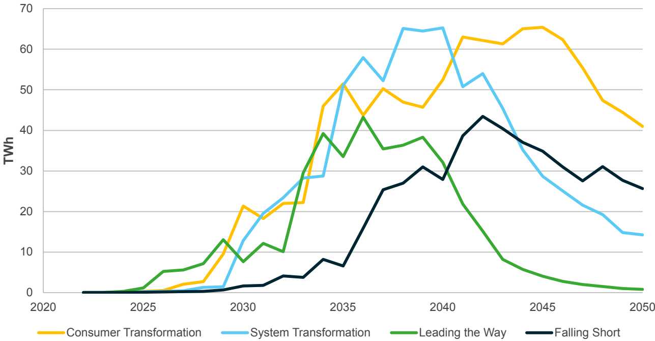
Figure FL.18: Annual curtailment (TWh) for all the scenarios out to 2050
