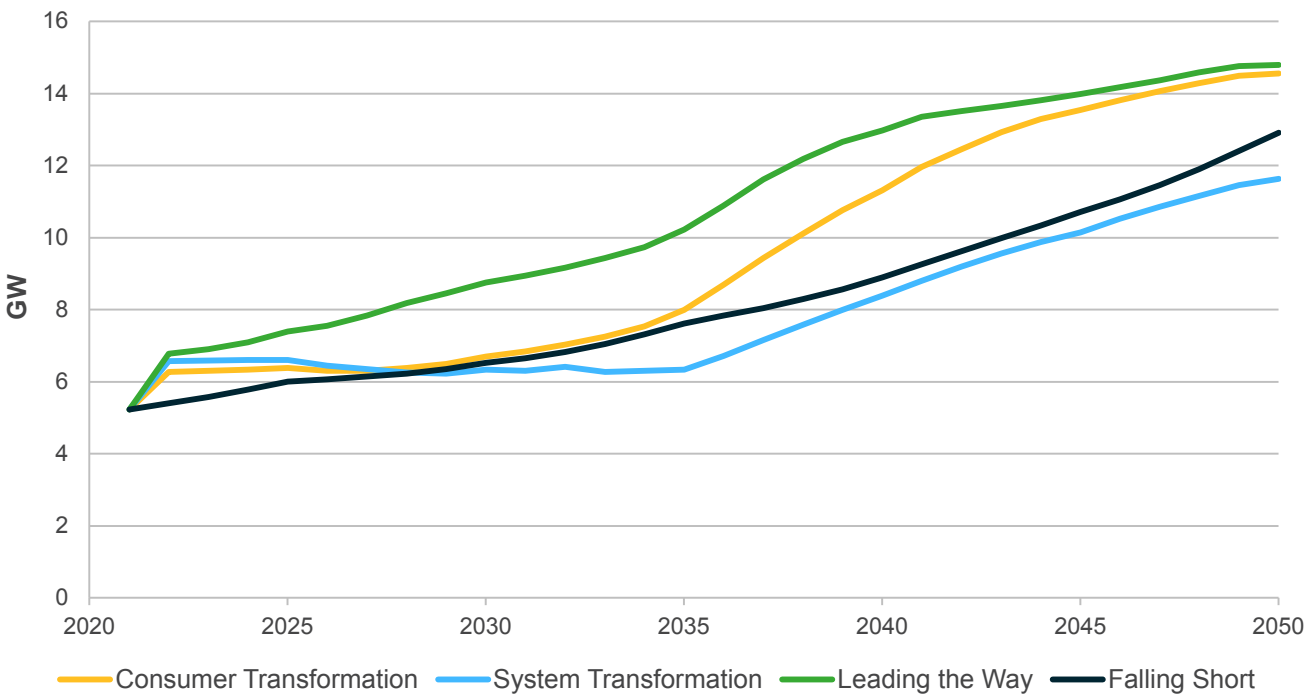
Figure FL.05: Total electric heat flexibility
