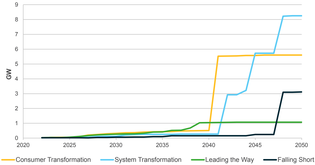
Figure ES.14: Marine capacity in GW
