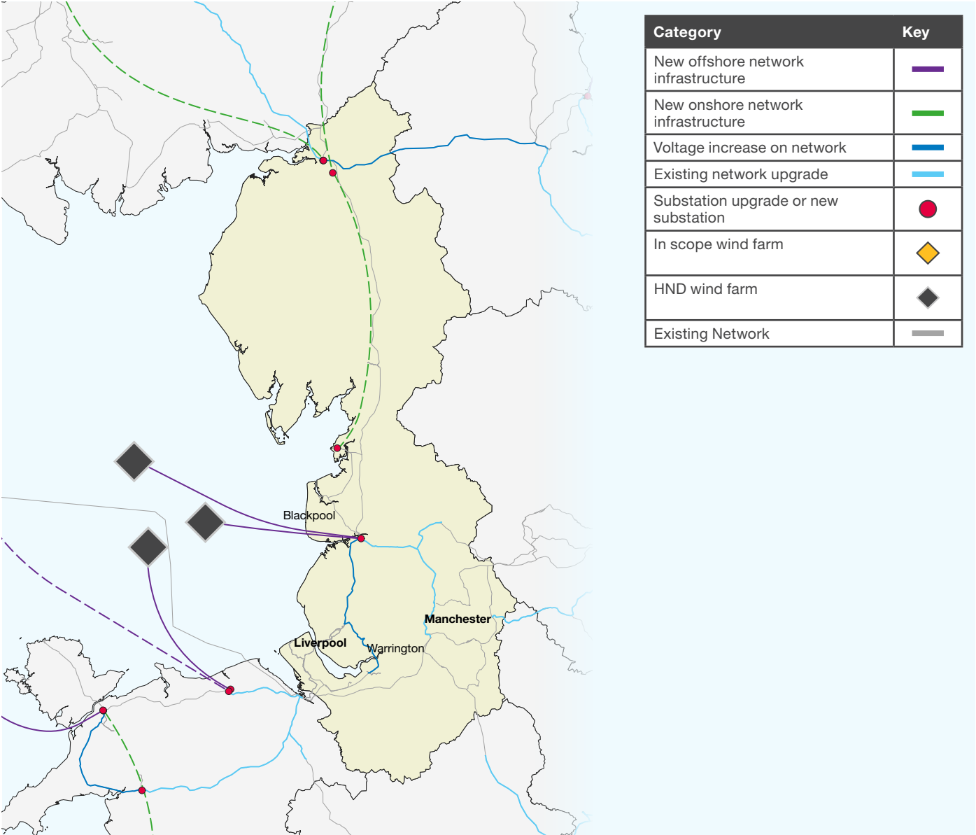
Figure 14. Map of all reinforcements in the North West region
