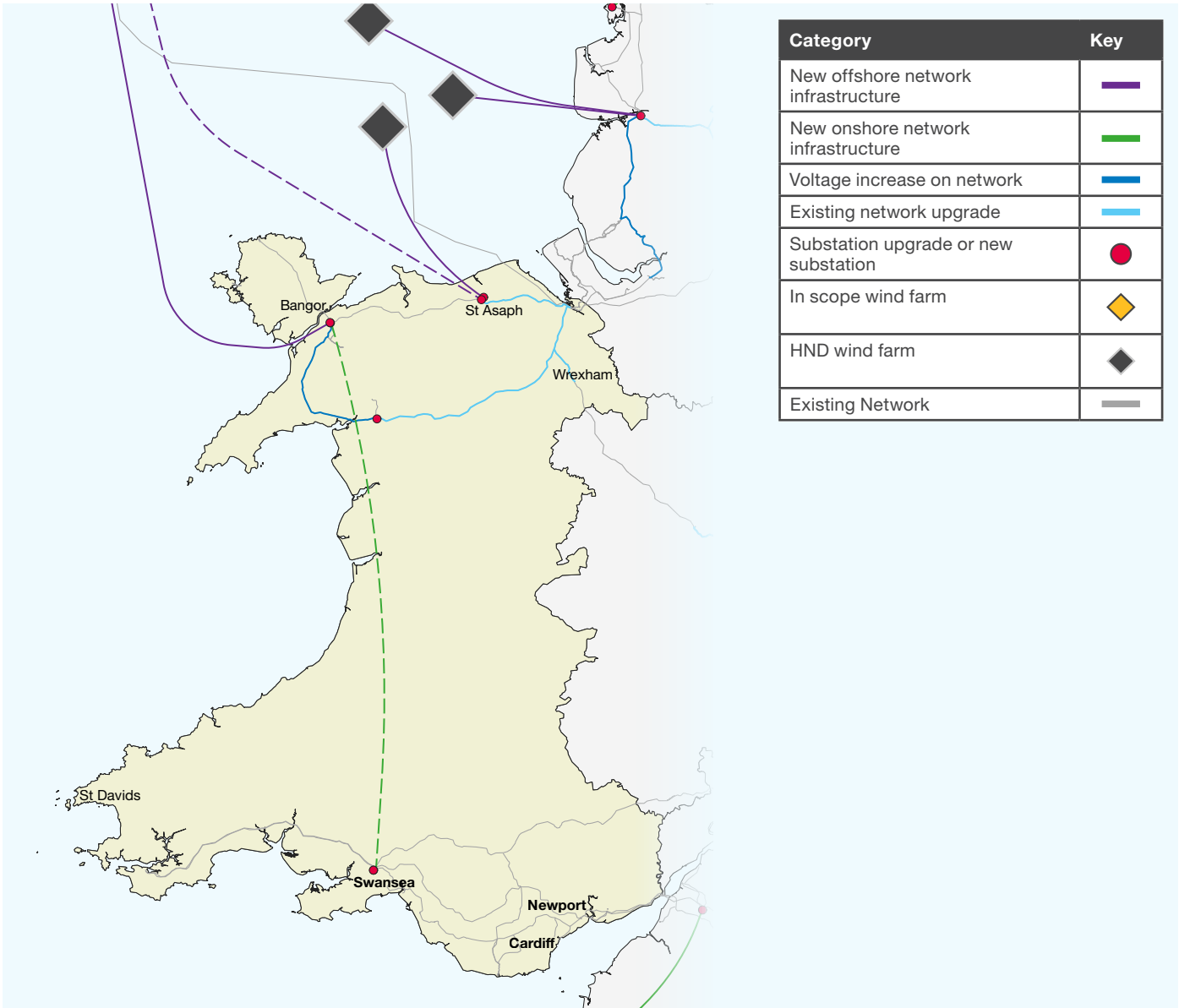
Figure 19. Map of all reinforcements in the Wales region *Dashed lines represent low maturity options Note: all routes and options shown on this map are for illustrative purposes only
