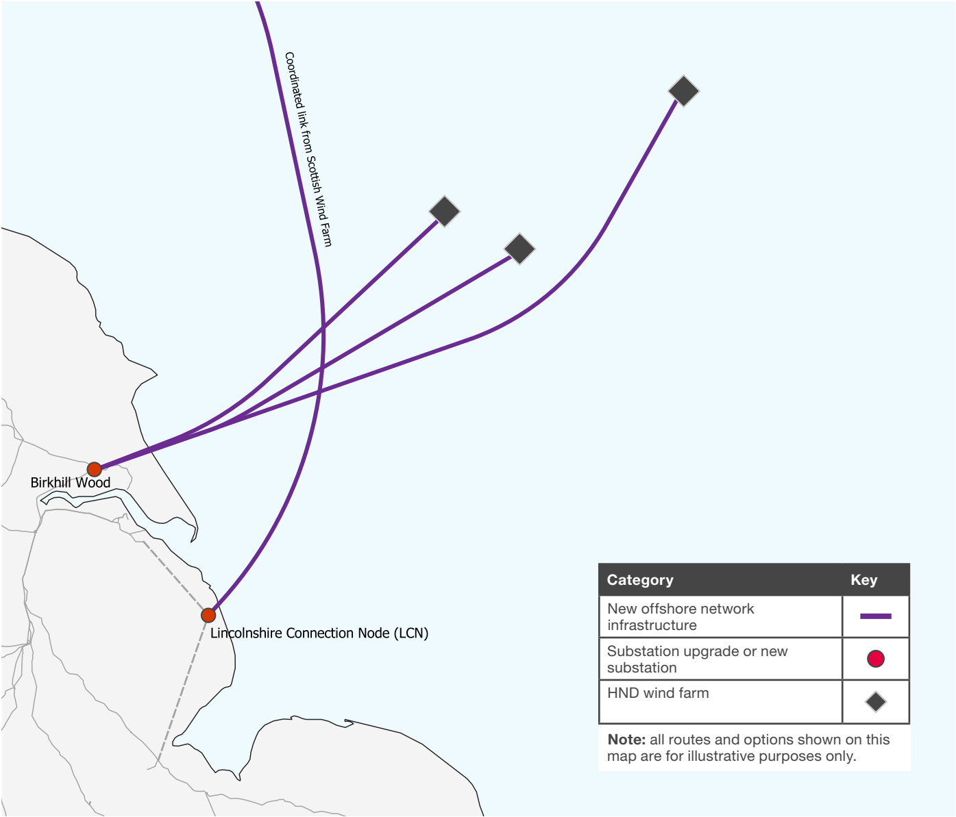
Figure 8. Map of new South Cluster design following Impact Assessment study
