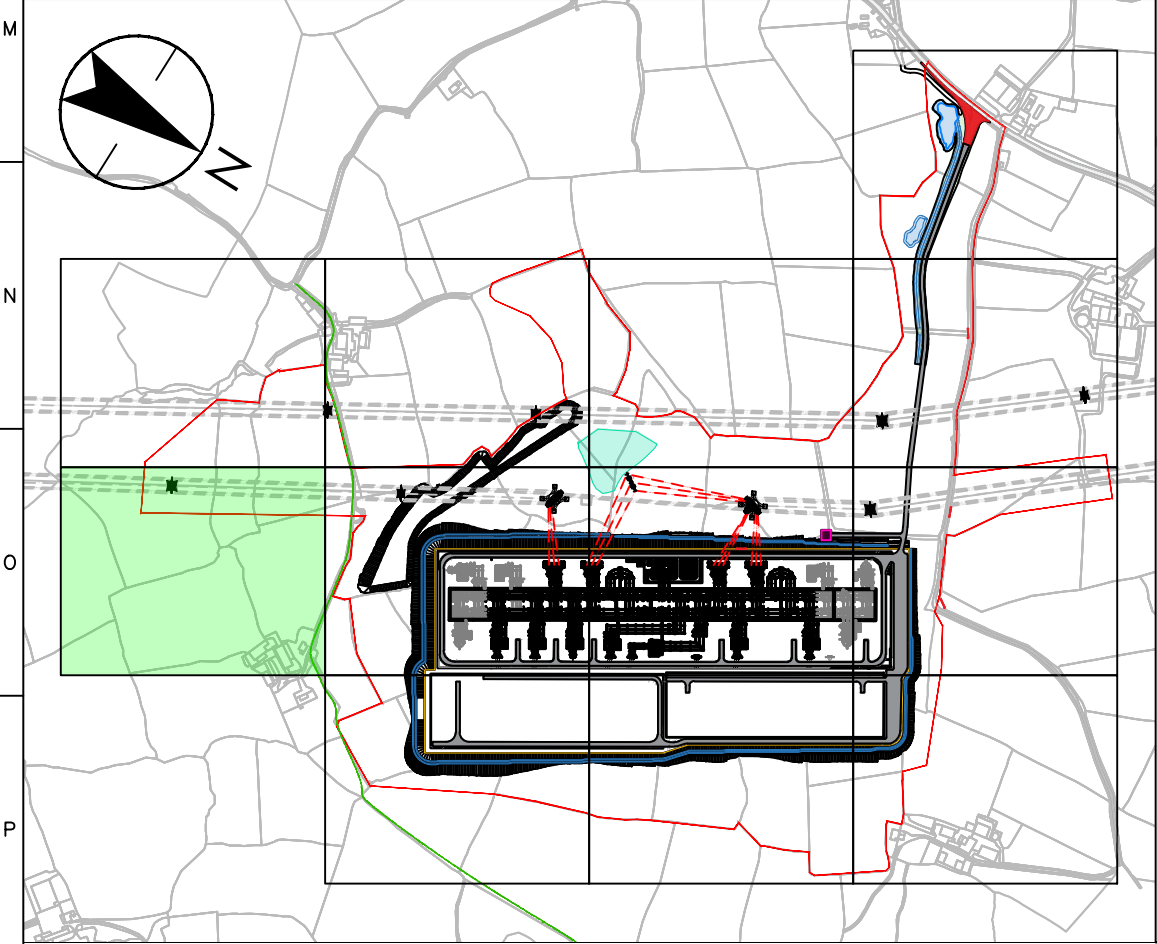
PROPOSED SITE KEY PLAN 1:10000 PROPOSED SITE LAYOUT PLAN - SHEET 6 1:500
