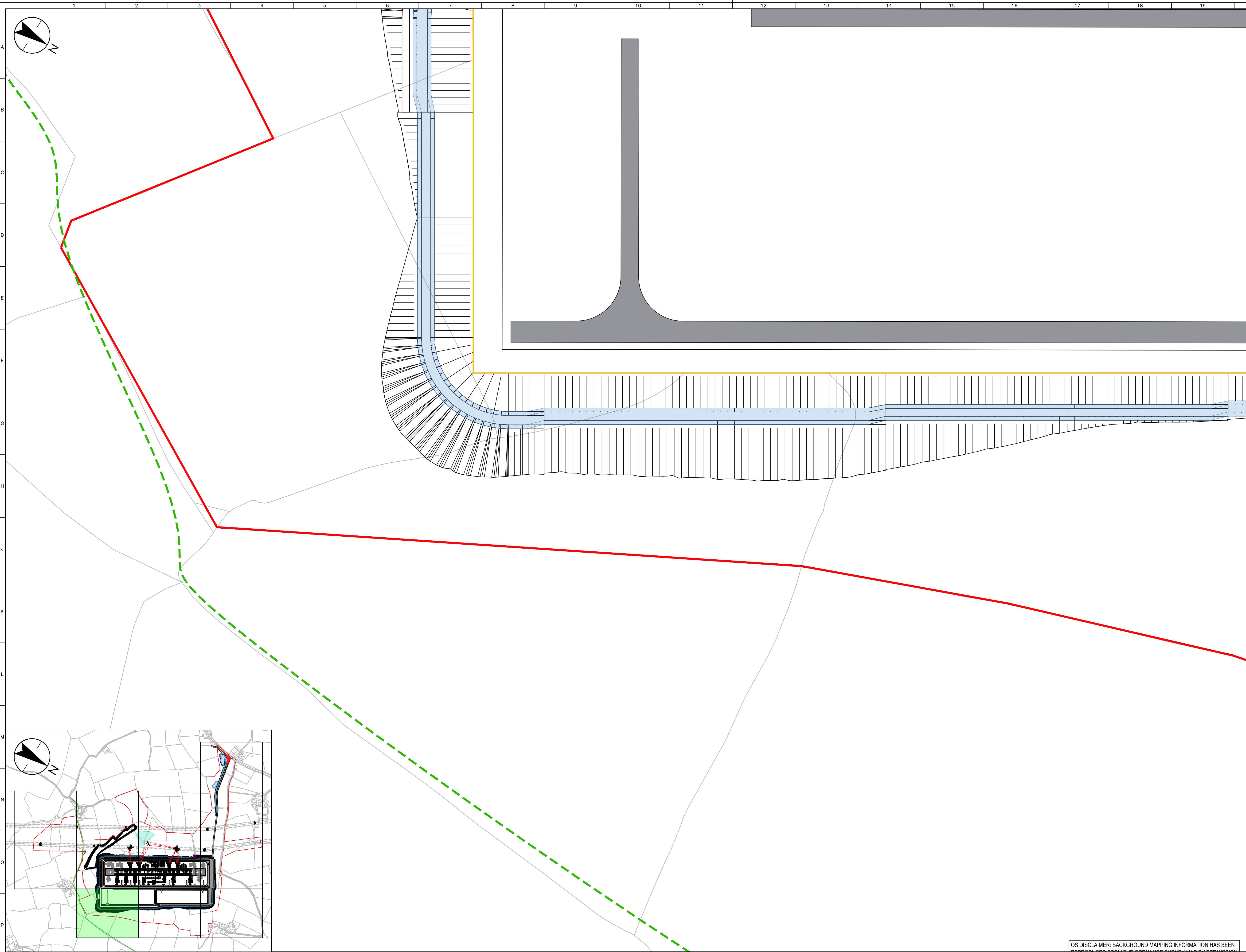
PROPOSED SITE LAYOUT PLAN - SHEET 10 1:500
