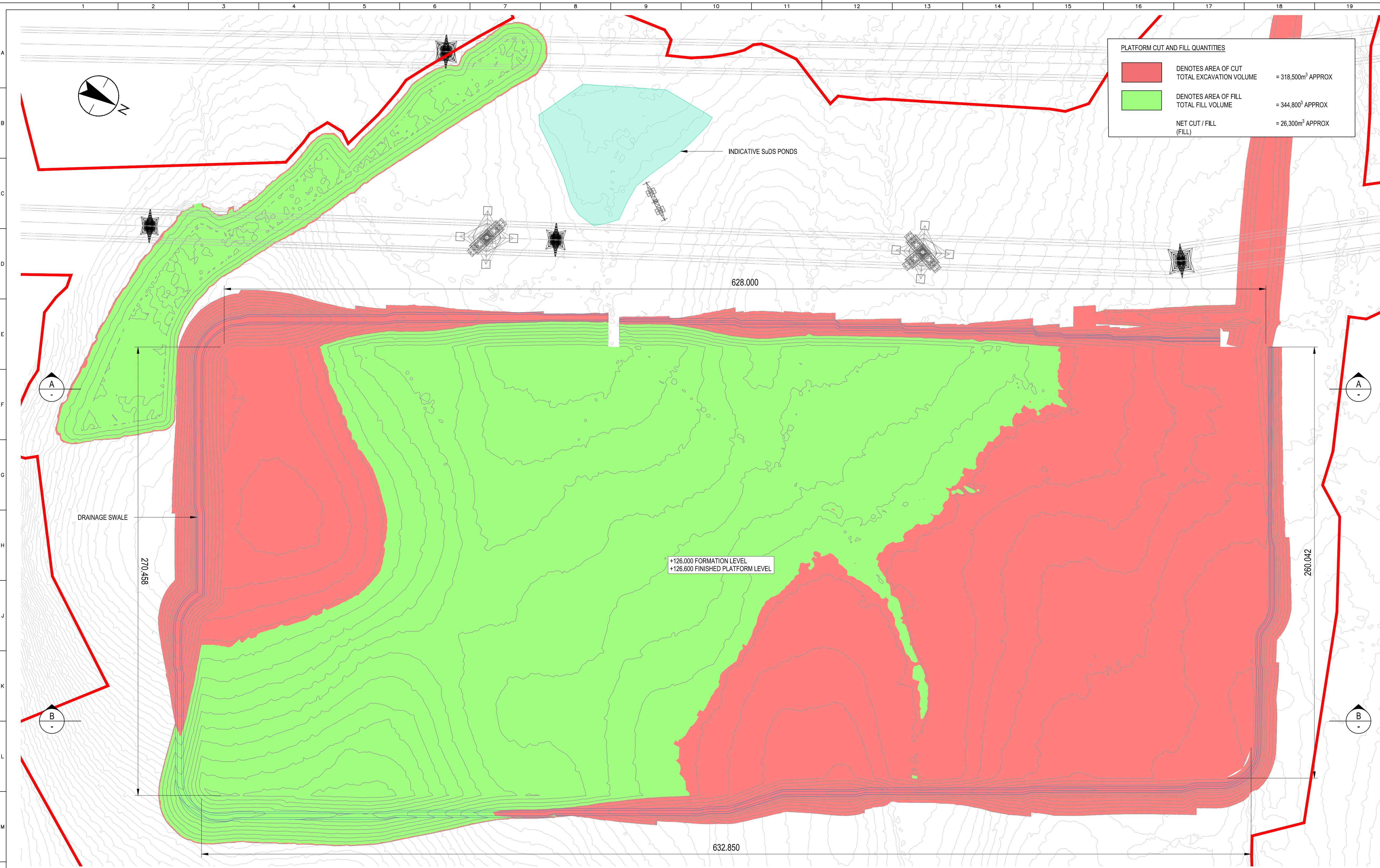
PLATFORM EARTHWORKS PLAN 1:1200
