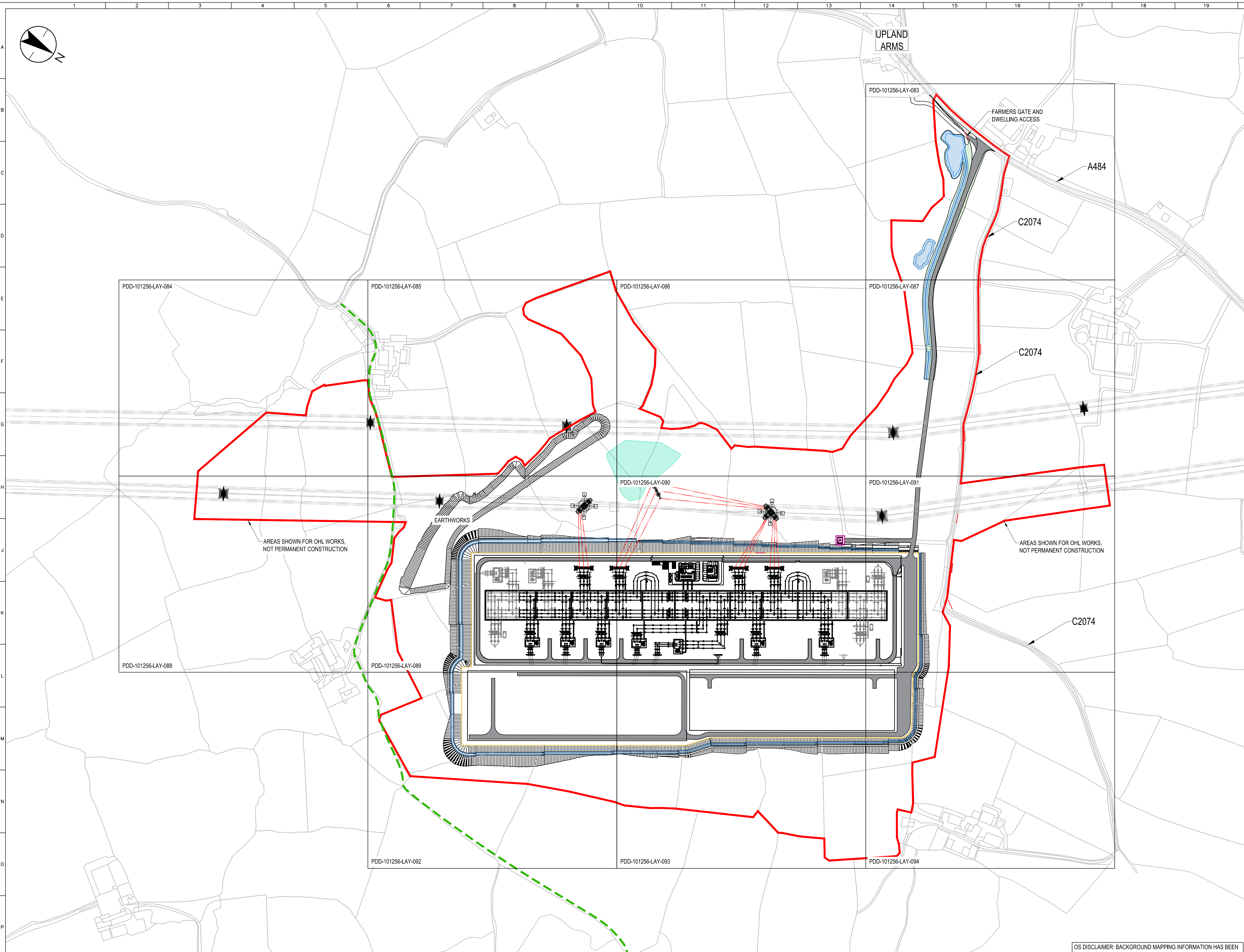
PROPOSED SITE LAYOUT PLAN - OVERALL LAYOUT 1:2500
