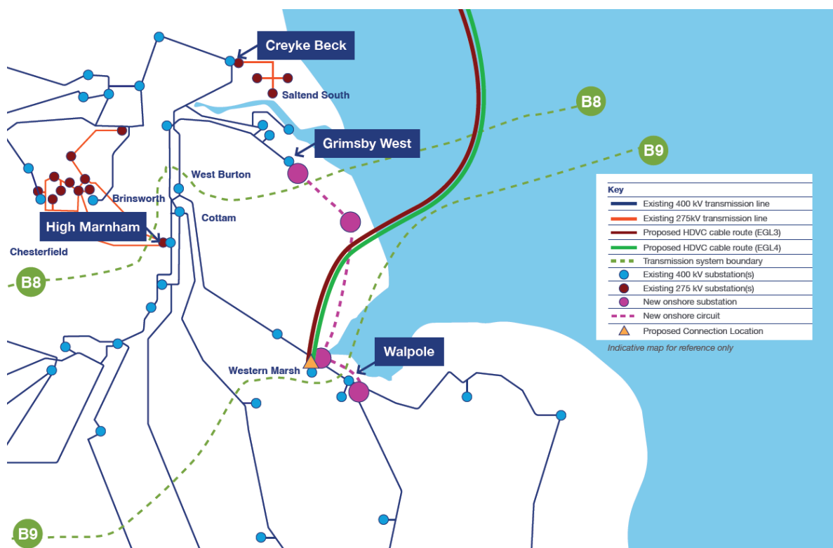
Figure 10.1 – EGL OPP4 New Weston Marsh potential strategic option
