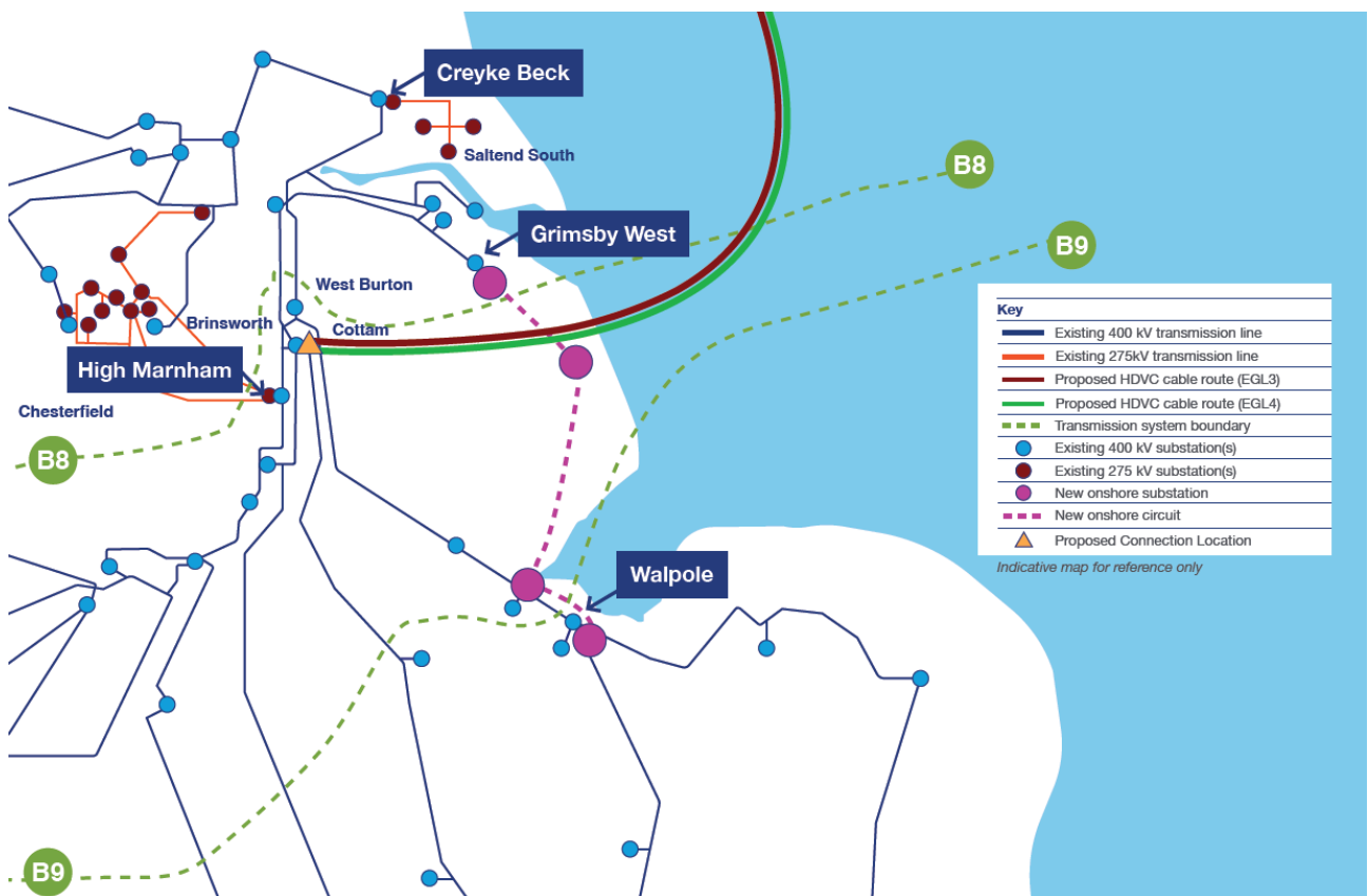
Figure 8.1 – EGL OPP2 Cottam potential strategic option
