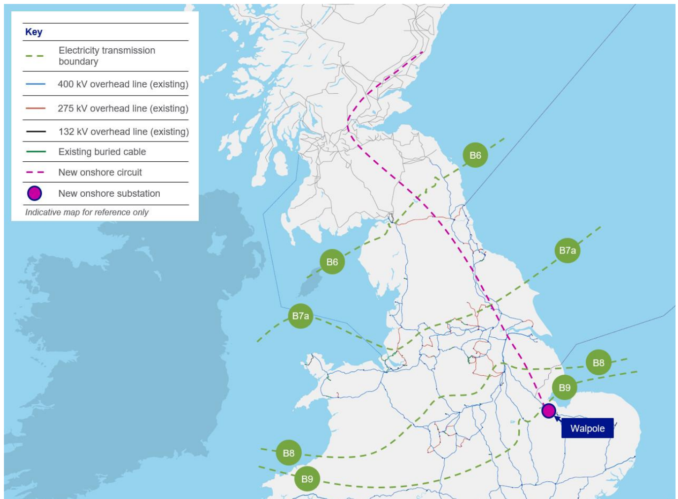
Figure F.1 – EGL OPP6 (land) New Walpole Substation
