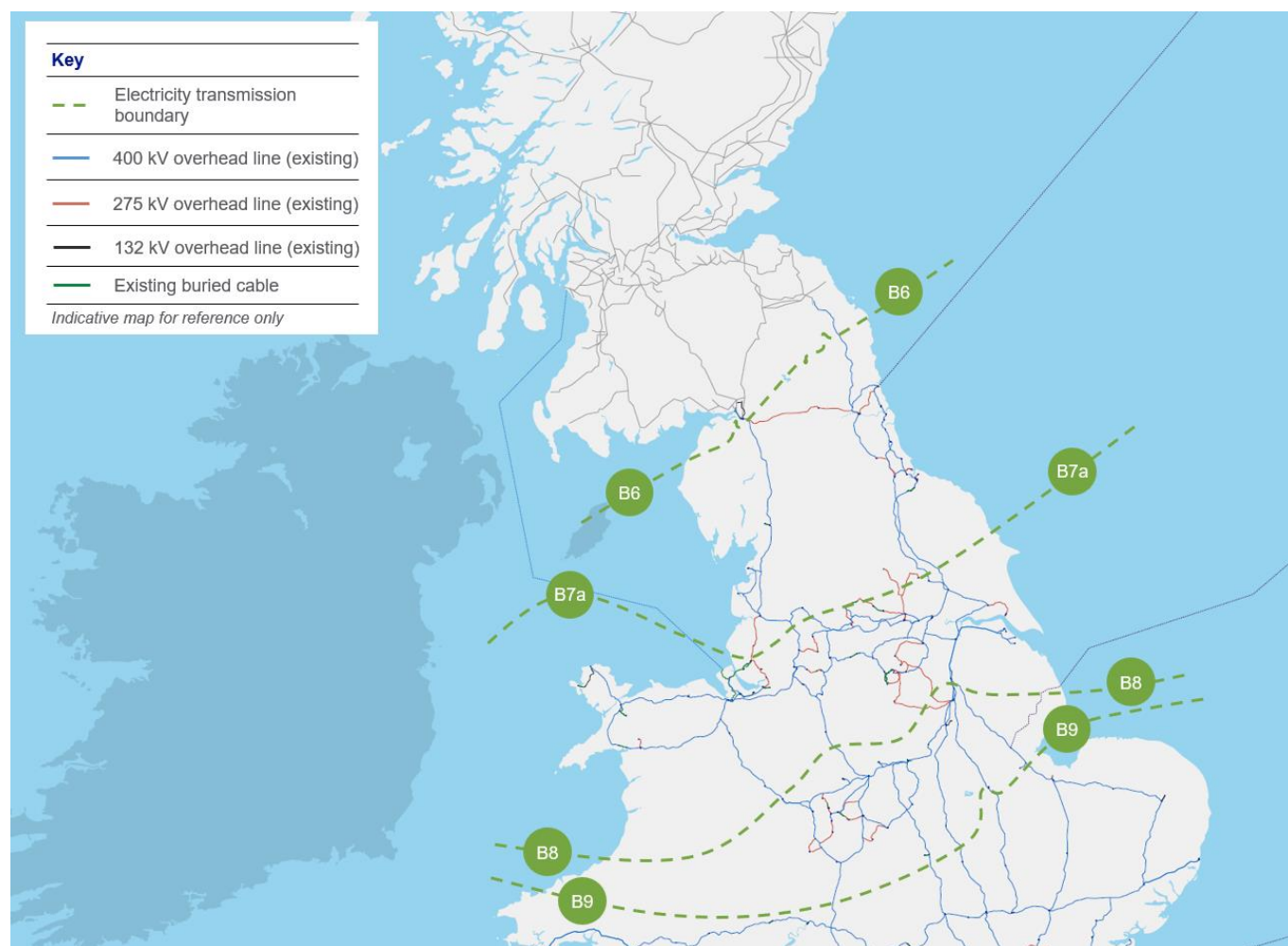
Figure B – Impacted Transmission Boundaries
