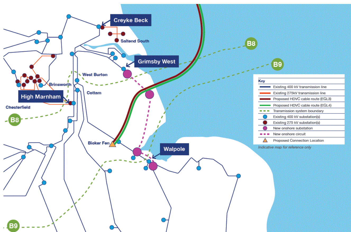
Figure 9.1 – EGL OPP3 Bicker Fen potential strategic option
