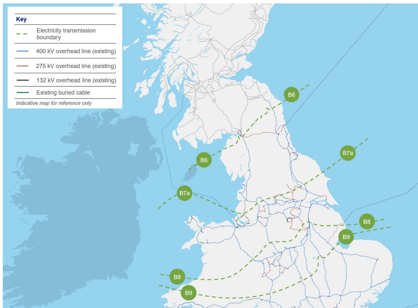
Figure 3.1 – The National Electricity Transmission System in Scotland, the North of England and the Midlands
