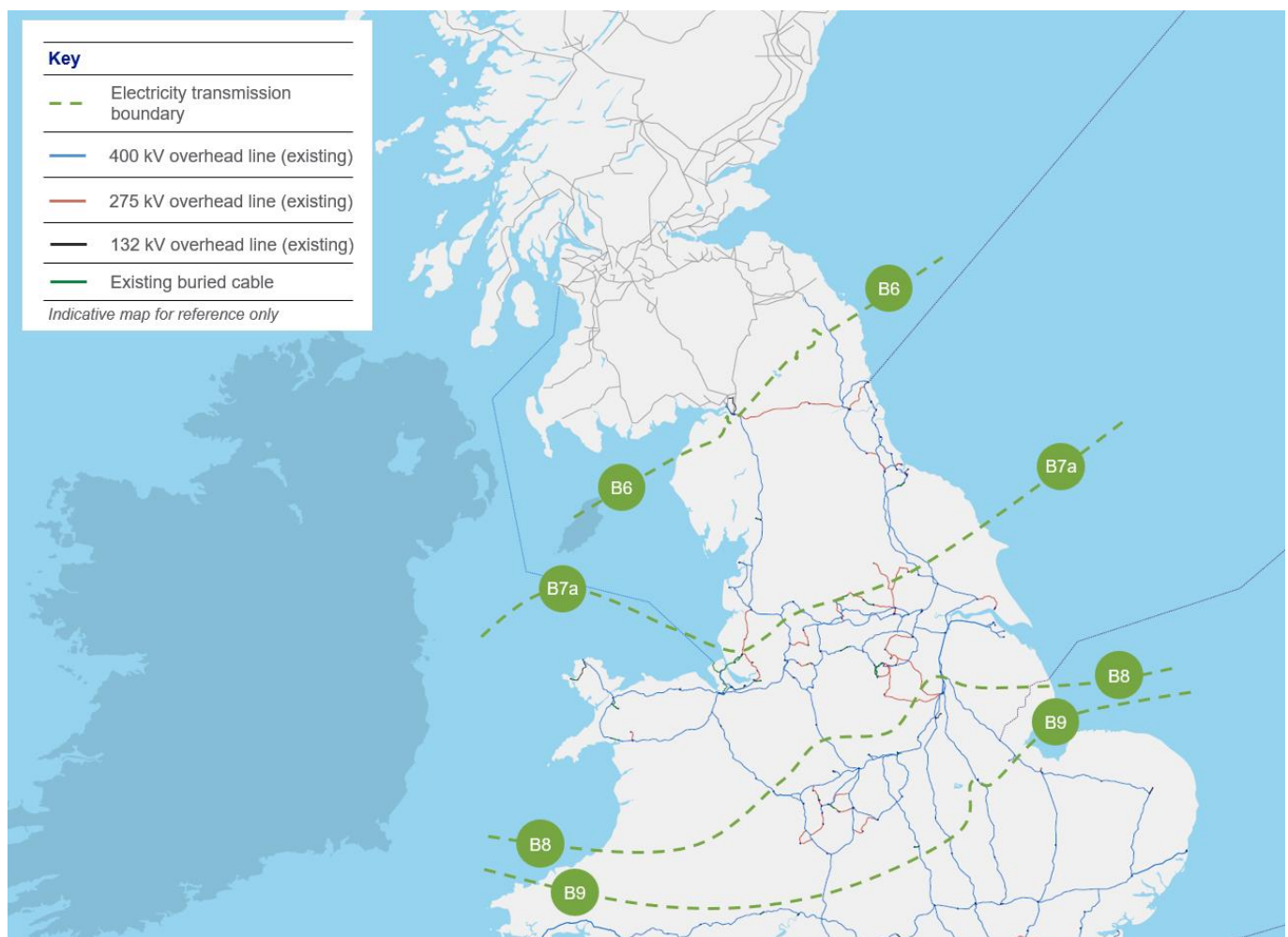
Figure 4.1 – The National Electricity Transmission System in Scotland, the North of England and the Midlands
