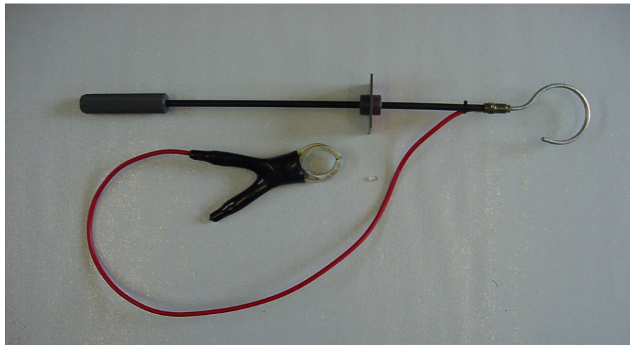
Figure 4.6B – Discharge Stick
