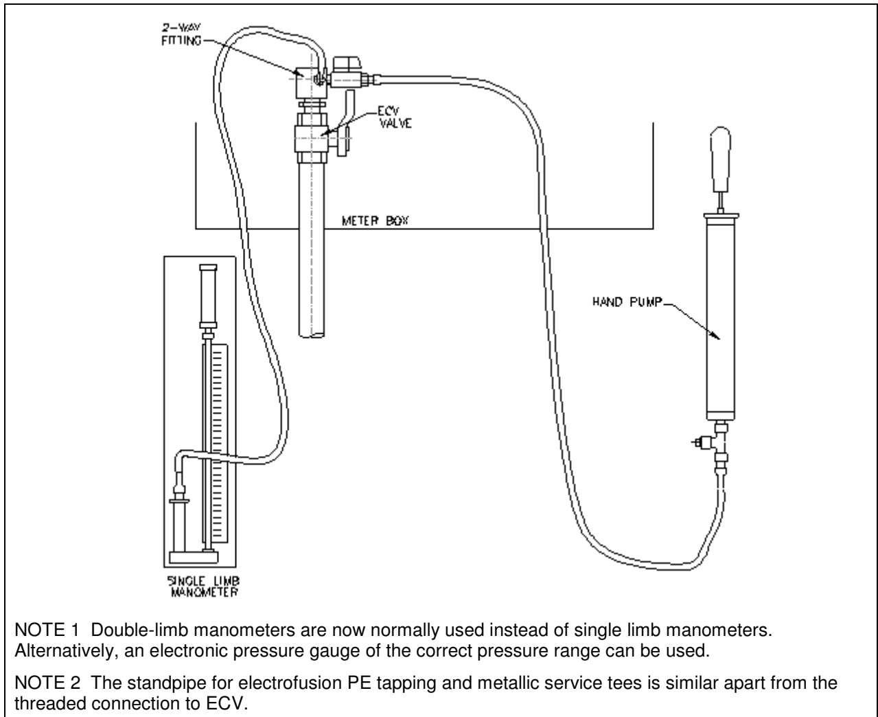
Figure A.2 — Typical test assembly for steel or polyethylene services from the house end using an emergency control valve
