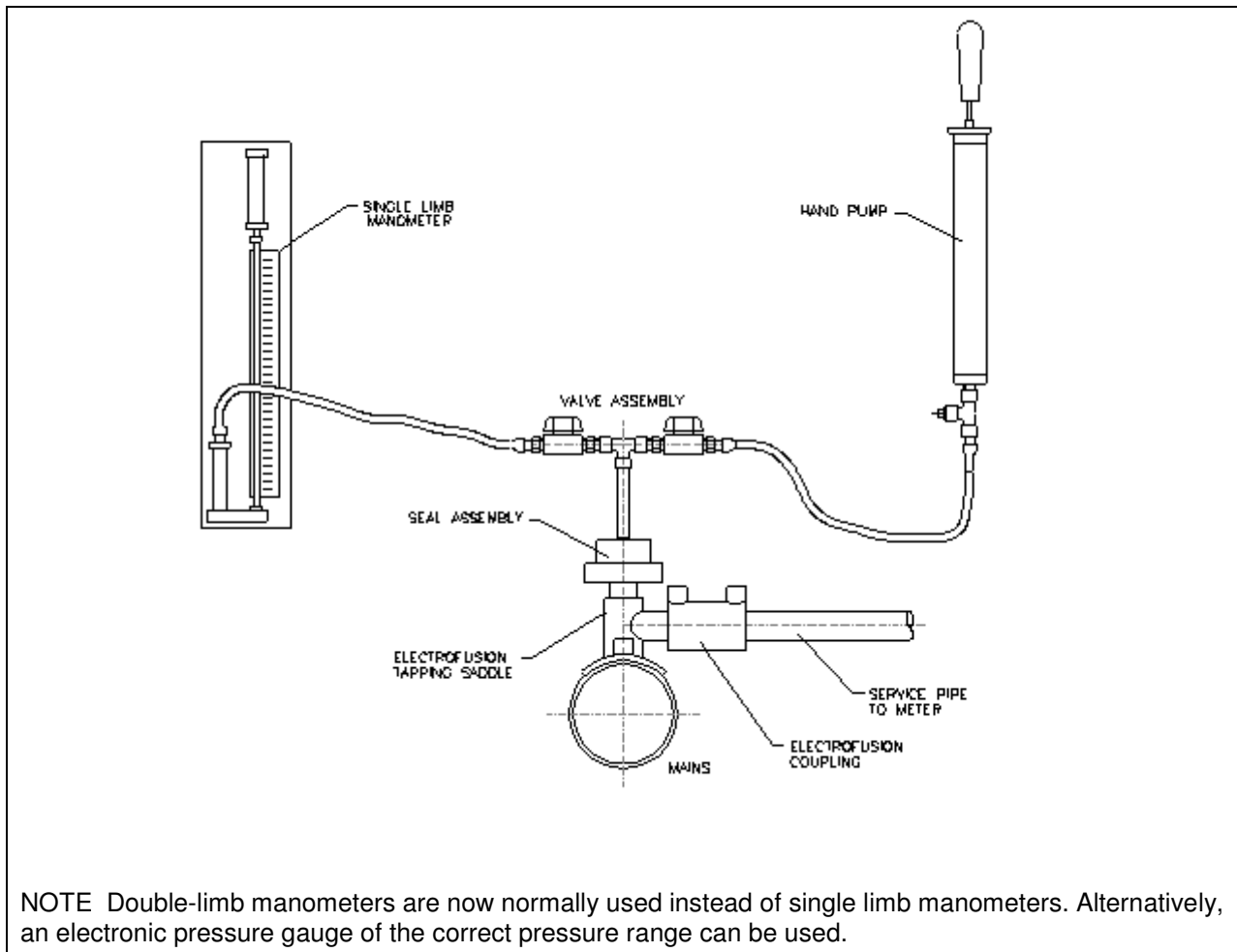
Figure A.3 — Typical test assembly for polyethylene service, top tee at the mains tapping end
