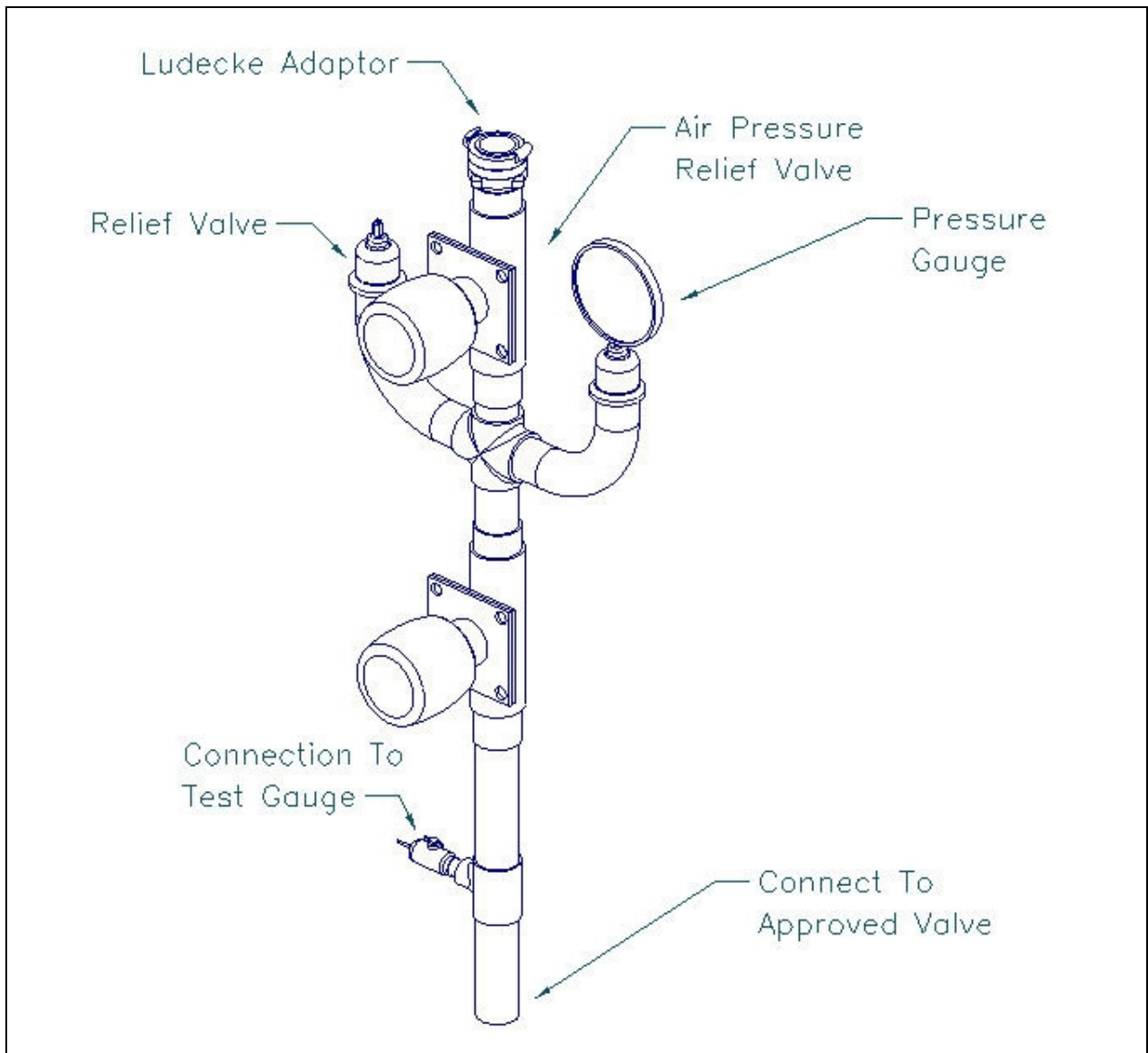
Figure A.1 — Typical test standpipe assembly for gas mains
