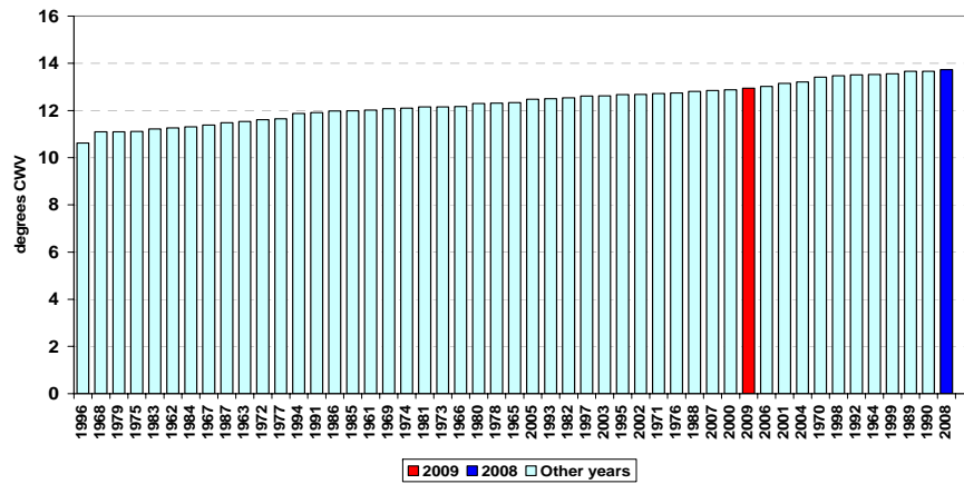
Mean National Composite Weather for May
