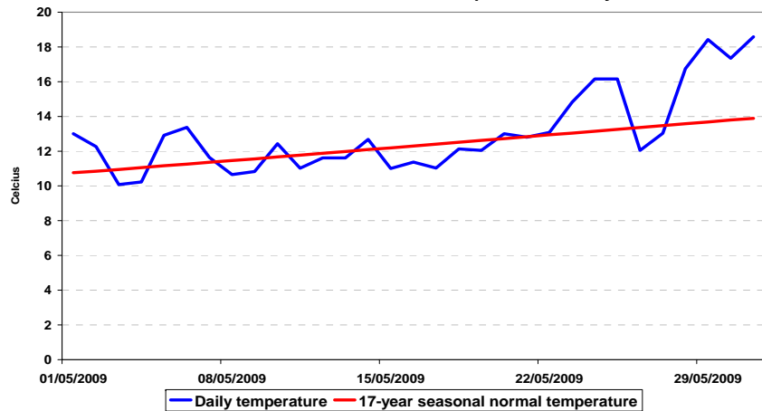
Actual and Seasonal Normal Temperature for May
