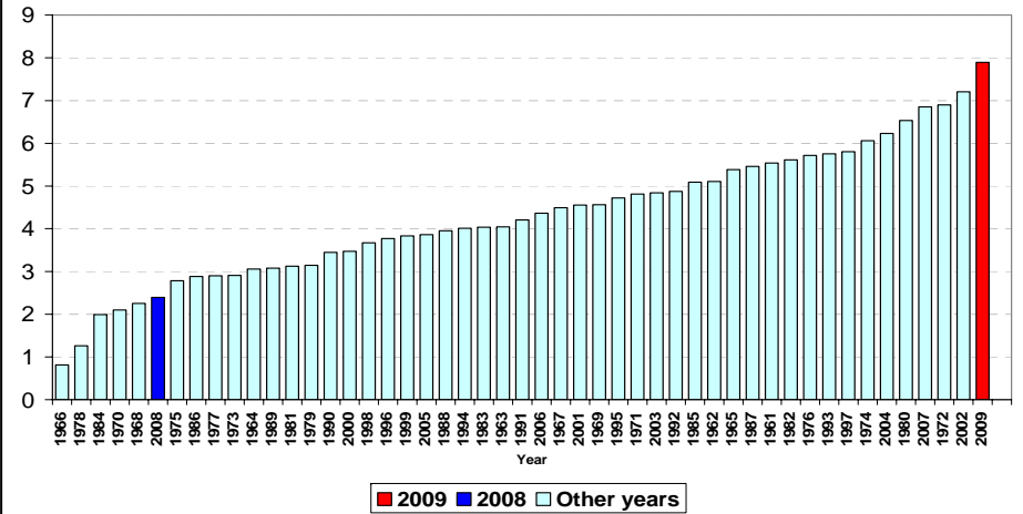
Minimum National Temperature for April
