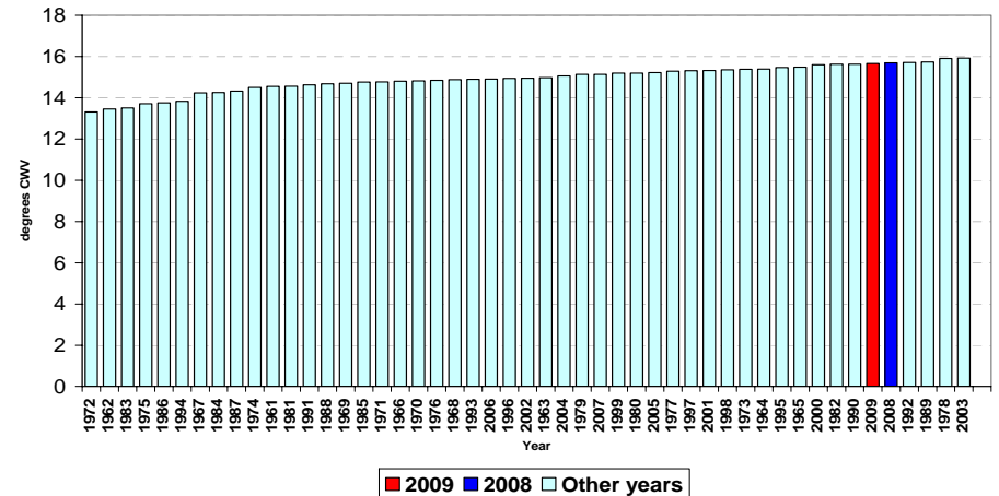
Maximum National Composite Weather for May
