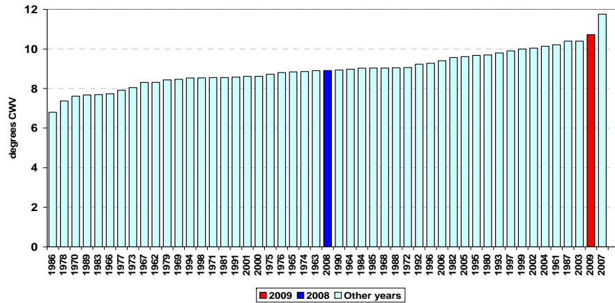
Mean National Composite Weather for April
