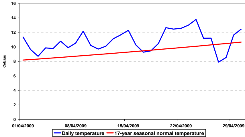
Actual and Seasonal Normal Temperature for April
