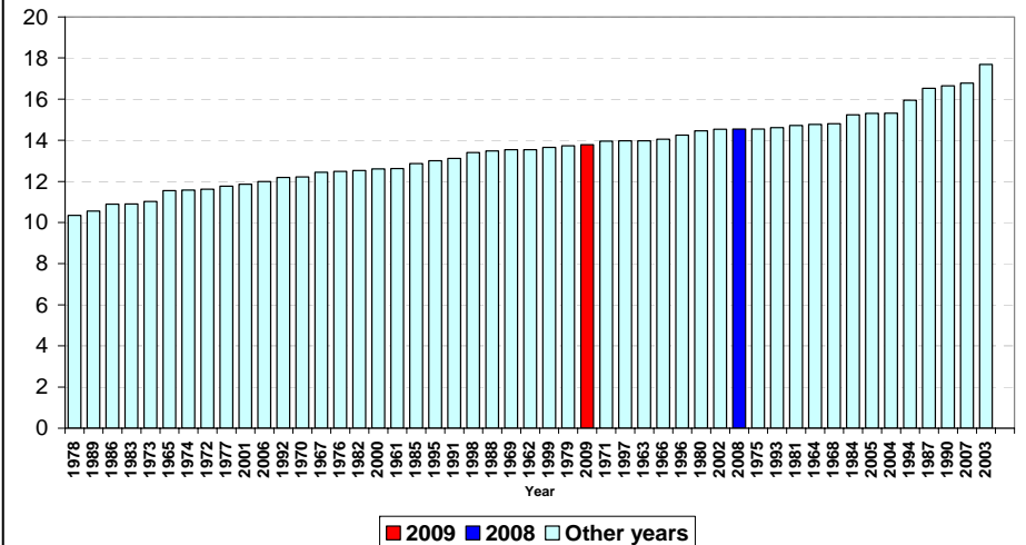
Maximum National Temperature for April
